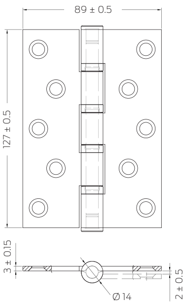
127mm/89mm/3mm, 4-ball bearings
