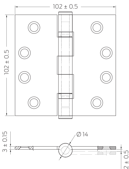
102mm/102mm/3mm, 2-ball bearings
