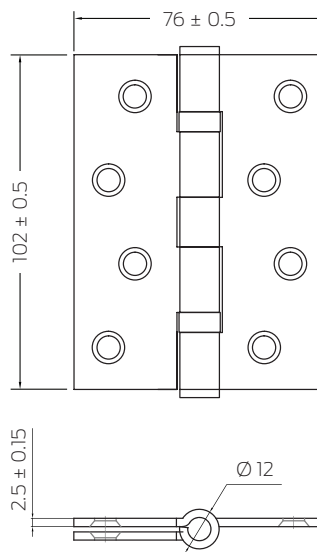
102mm/76mm/2.5mm, 2-ball bearings
