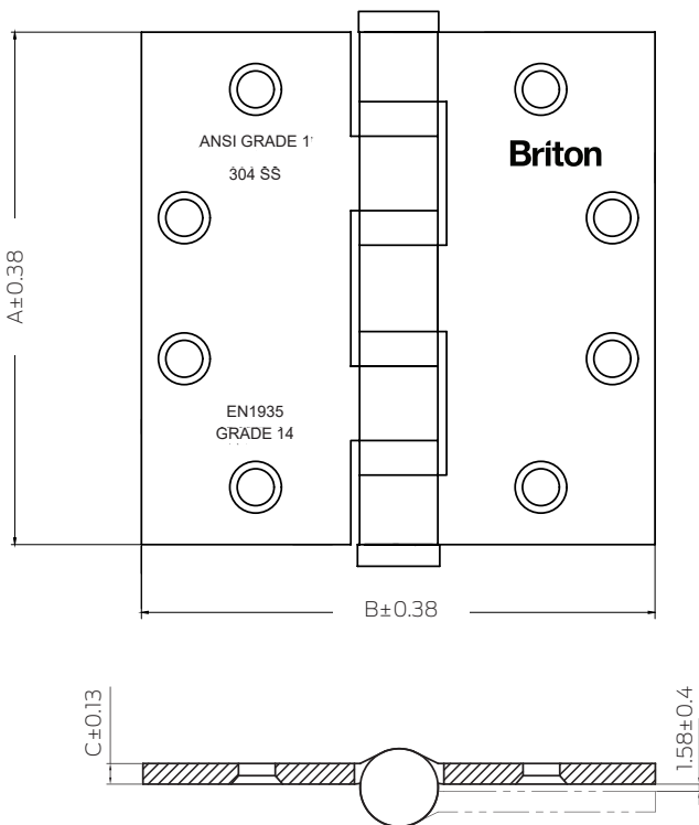
AH500HW series hinge, 4 ball bearings
