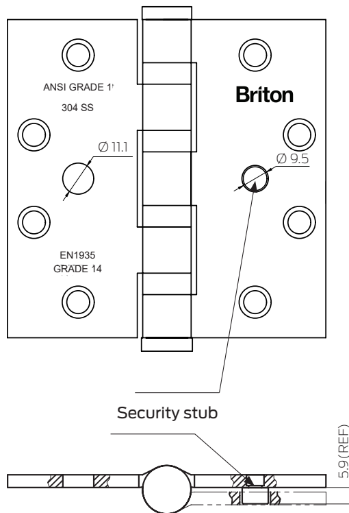
AH500HW series hinge, 4 ball bearings, with security stub
